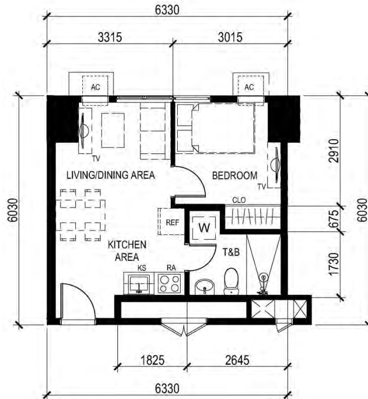
UNIT 22 (12 th , 22 nd , 32 nd level) 35.25 SQ.M.
