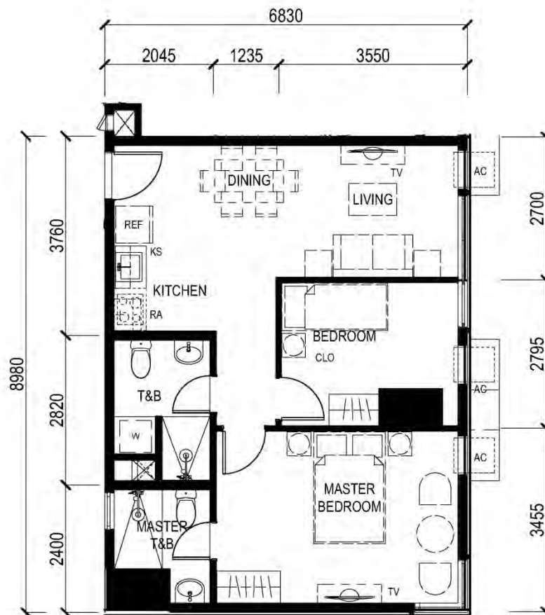
UNIT 01 (45 th level) 61.76 SQ.M.
