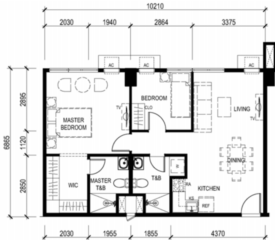
UNIT 07 (45 th level) 70.19 SQ.M.
