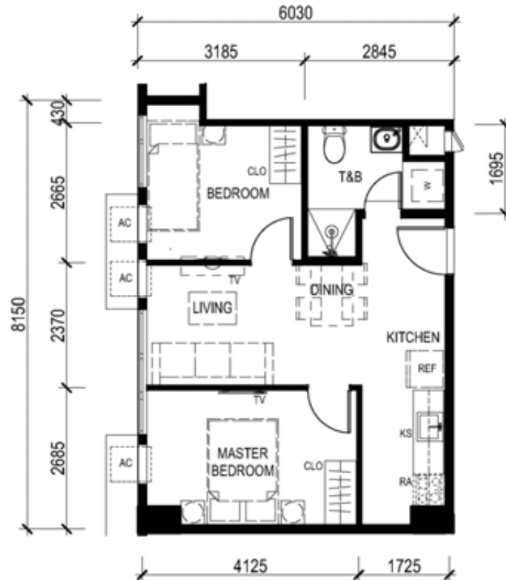
UNIT 04 (45 th level) 47.37 SQ.M.
