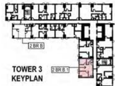
UNIT 02 (45 th level) 48.78 SQ.M.
