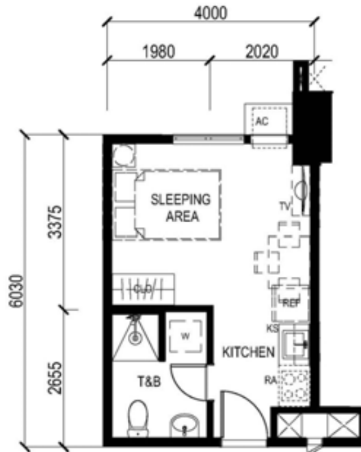
UNIT 11 (4 th to 6 th level) UNIT 09 (7 th to 8 th level) UNIT 18 (9 th to 44 th level) 24.12 SQ.M.
