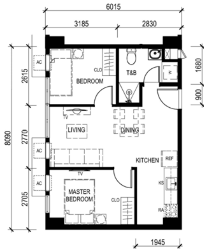
UNIT 02 (45 th level) 48.78 SQ.M.
