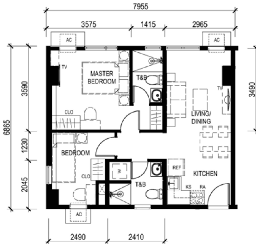
UNIT 11 (45 th level) 55.11 SQ.M.
