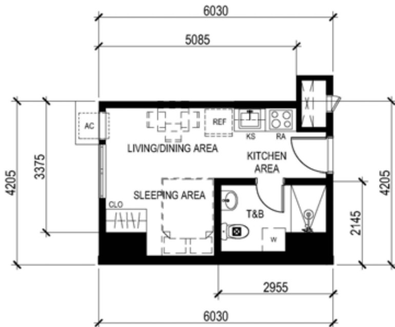
UNIT 03 (9 th to 44 th level) 24.81 SQ.M.
