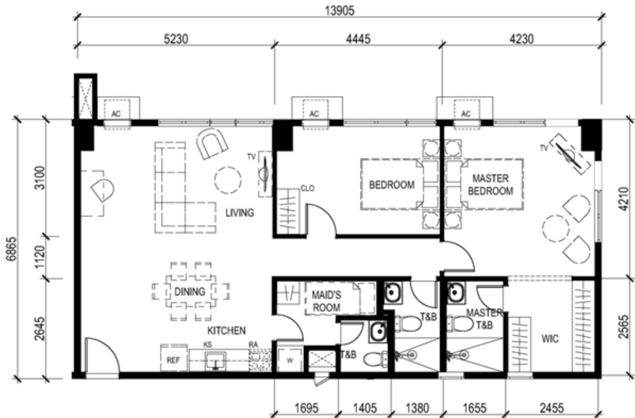
UNIT 05 (45 th level) 95.46 SQ.M.
