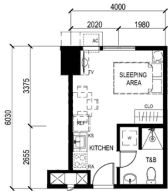
UNIT 12 (4 th to 6 th level) UNIT 10 (7 th to 8 th level) UNIT 20 (9 th to 44 th level) 24.12 SQ.M.
