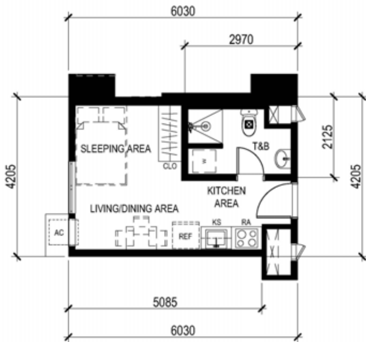
UNIT 01 (4 th to 6 th level) UNIT 01 (9 th to 44 th level) 28.17 SQ.M.
