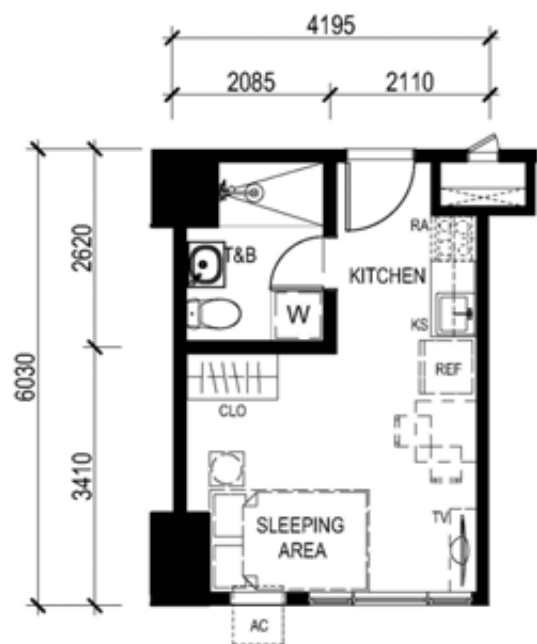
UNIT 19 (9 th to 44 th level) 24.12 SQ.M.
