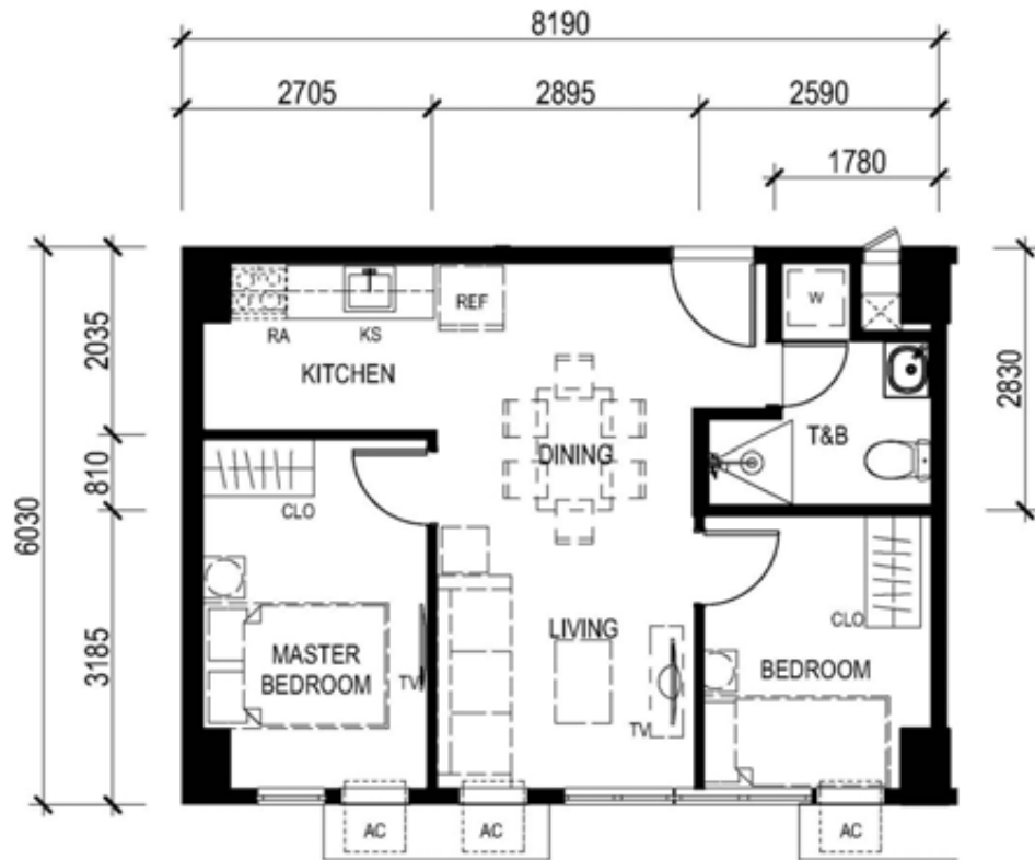
UNIT 10 (45 th level) 49.39 SQ.M.
