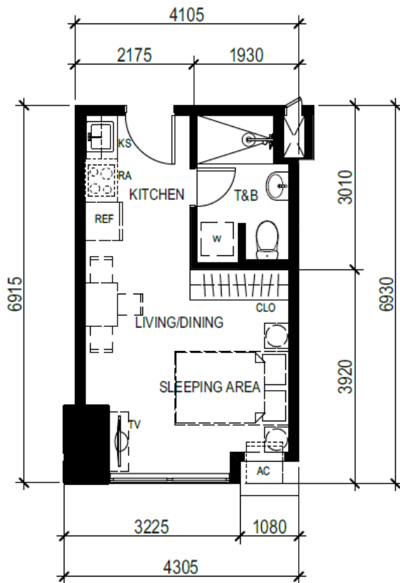
UNIT 3 (5 th to 6 th level) UNIT 4 (7 th to 44 th level) 27.27 SQ.M.
