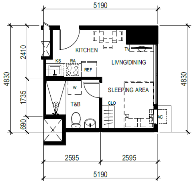
UNIT 09 (7 th to 8 th level) UNIT 16 (9 th to 44 th level) 24.79 SQ.M.
