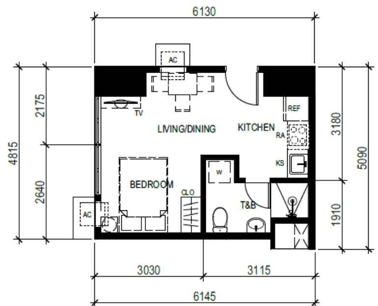
UNIT 8 (8 th to 44 th level) 29.08 SQ.M.
